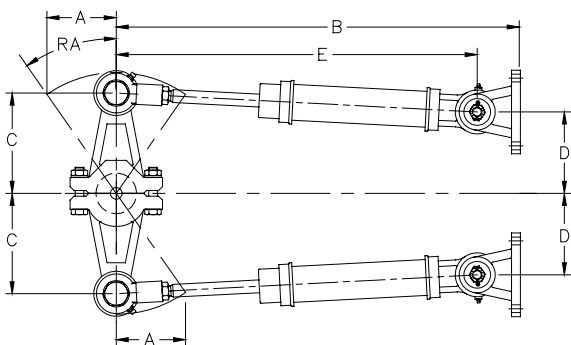
DIE CAST UNBALANCED CYLINDERS – RUDDER ANGLE (RA) 35°
