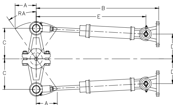
UNBALANCED CYLINDERS – RUDDER ANGLE (RA) 35°
