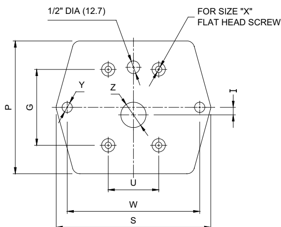
FRONT MOUNTING PLATE (OPTIONAL)
